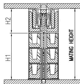
MATING HEIGHT
